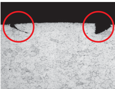
Cracks shown in cross-section. Such surface defects are usually already present prior to forming.
