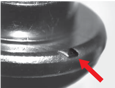
Profile crack
